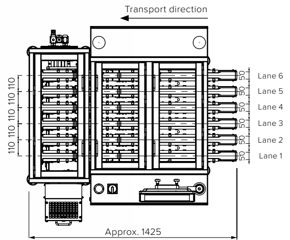
All entries in mm | Drawing shows sample version
