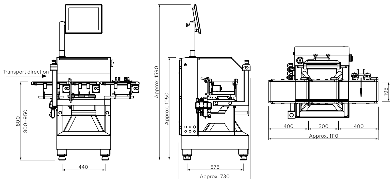
State-of-the-art HC-A weighing technology as multi-track option
